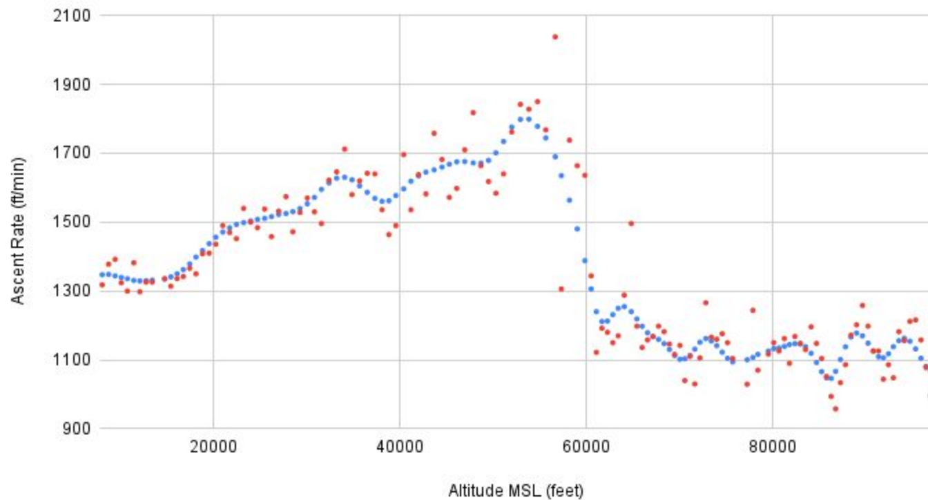
264846_6 Ascent Rate vs Altitude (77.8 rms difference)
