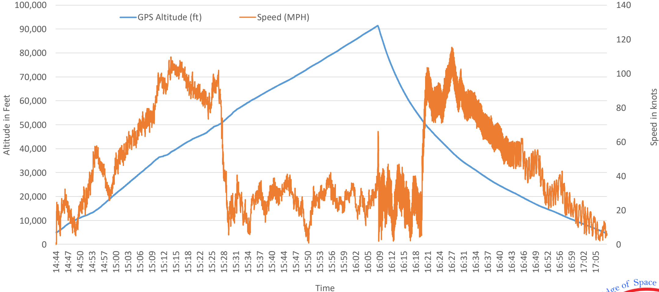
Speed vs Altitude
