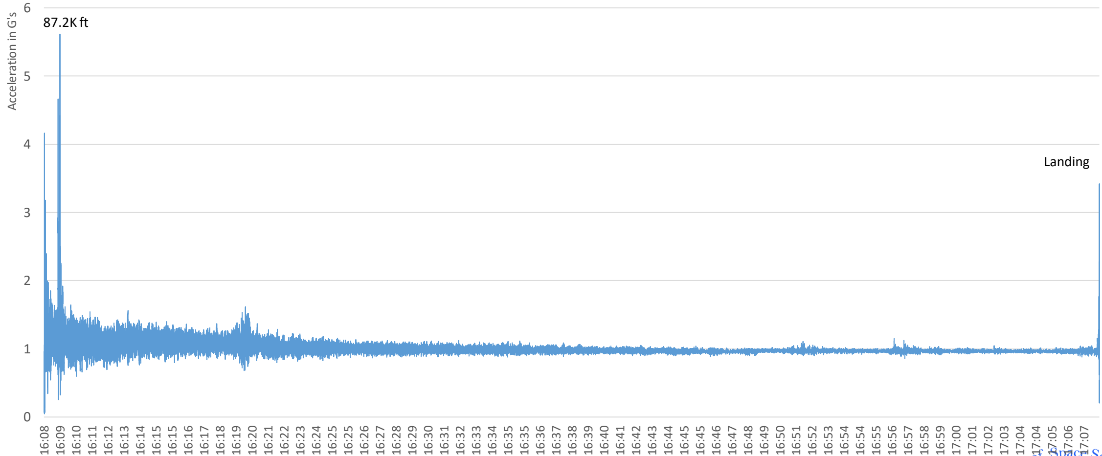
Acceleration: Burst to Landing
